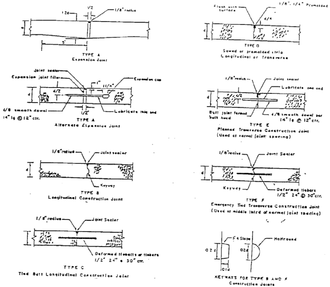
FIGURE 4.5 TYPICAL JOINT DETAILS
