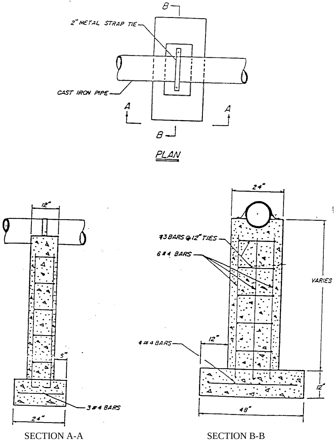
FIGURE 5.6 TYPICAL PIER DETAIL
