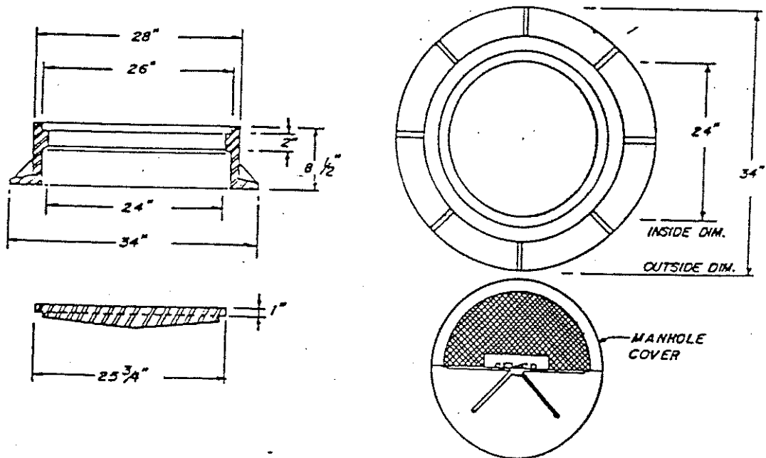
MANHOLD DETAIL
