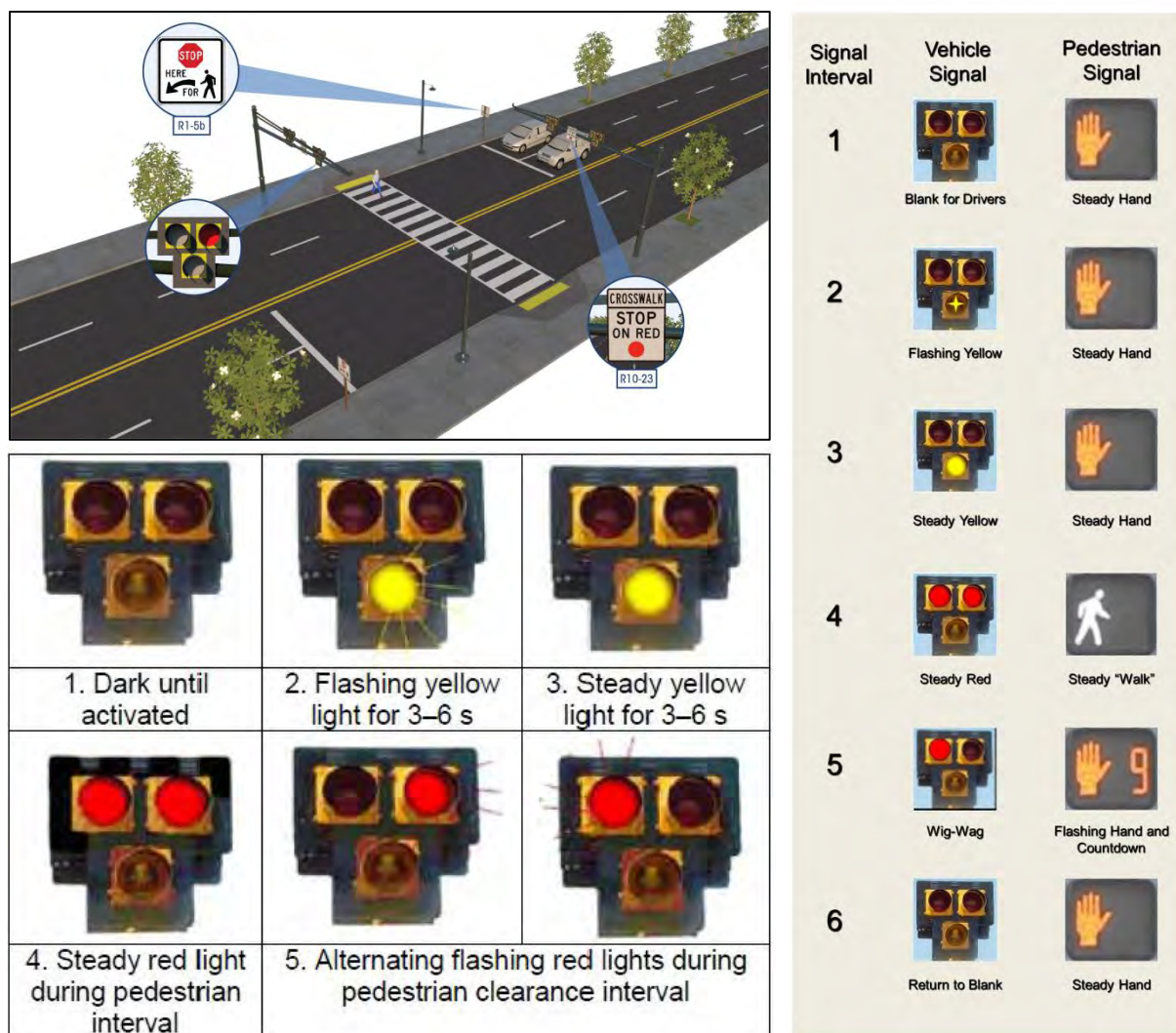
Figure 66: Pedestrian Hybrid Beacon Layout, Display, and Operation Example (Source: PEDSAFE)
