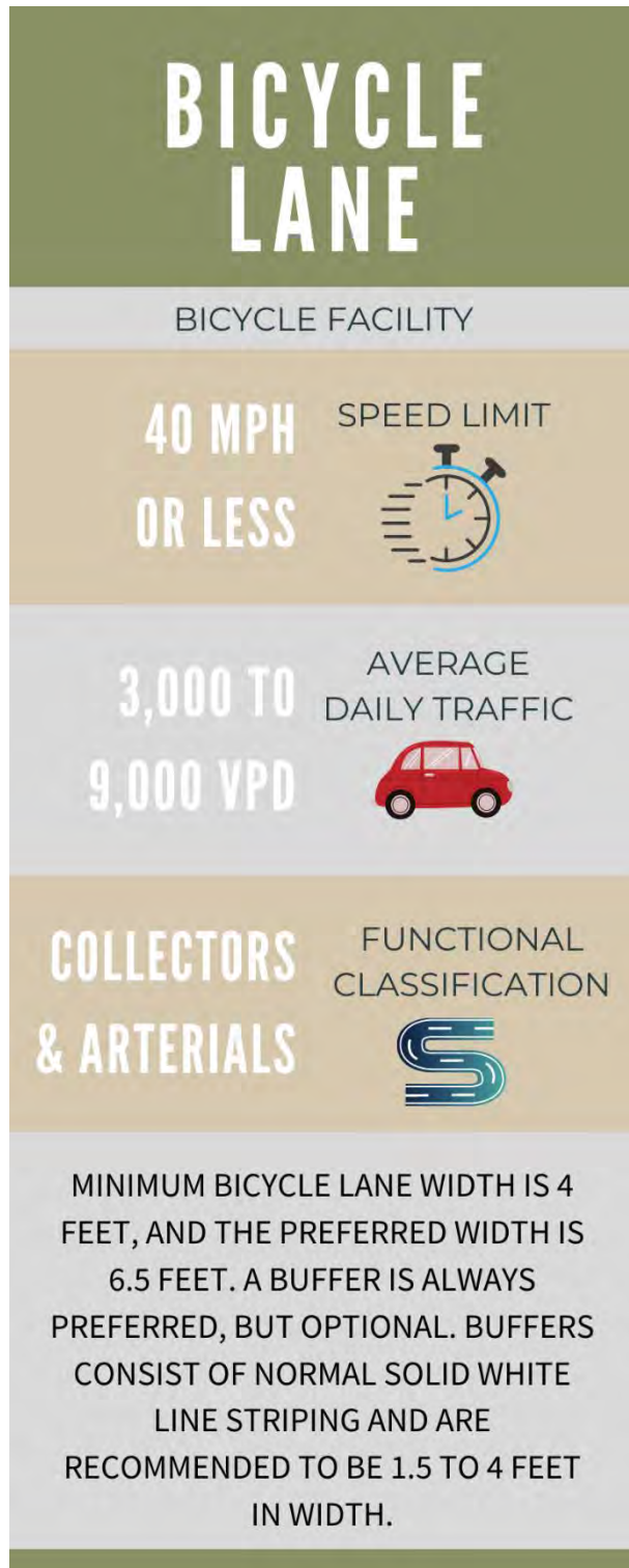
Figure 45: Bicycle Lane Guidance
