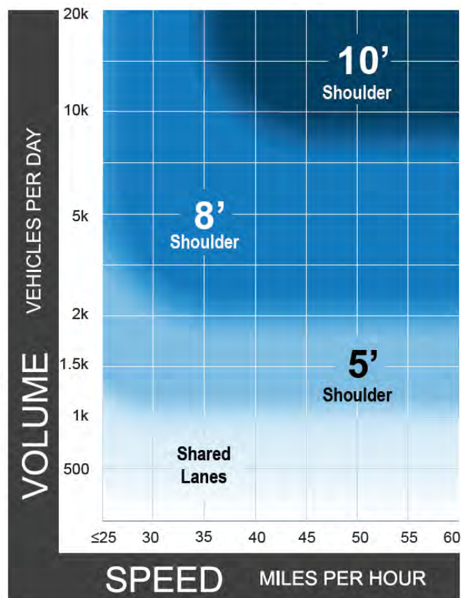
Figure 40: Preferred Shoulder Widths for Rural Roadways (Source: FHWA)
