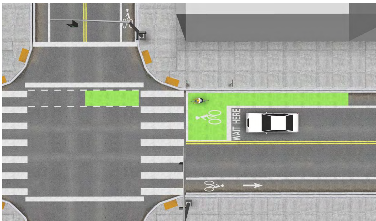
Figure 57: Bike Box Example (Source: NACTO)
