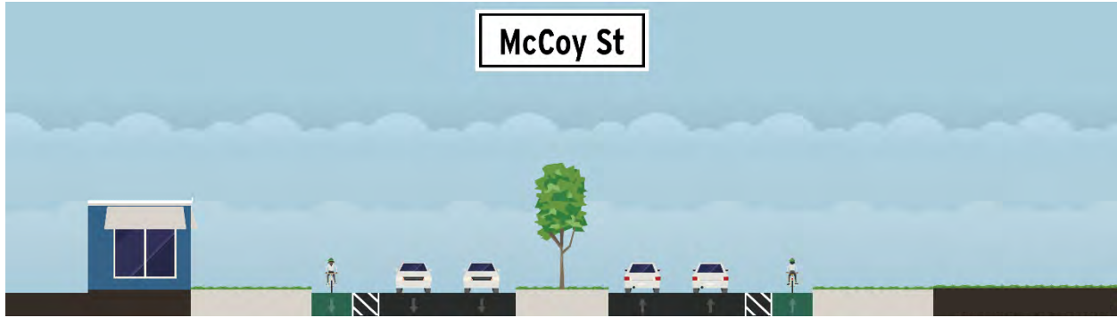
Figure 33: Proposed Typical Section for McCoy Street
