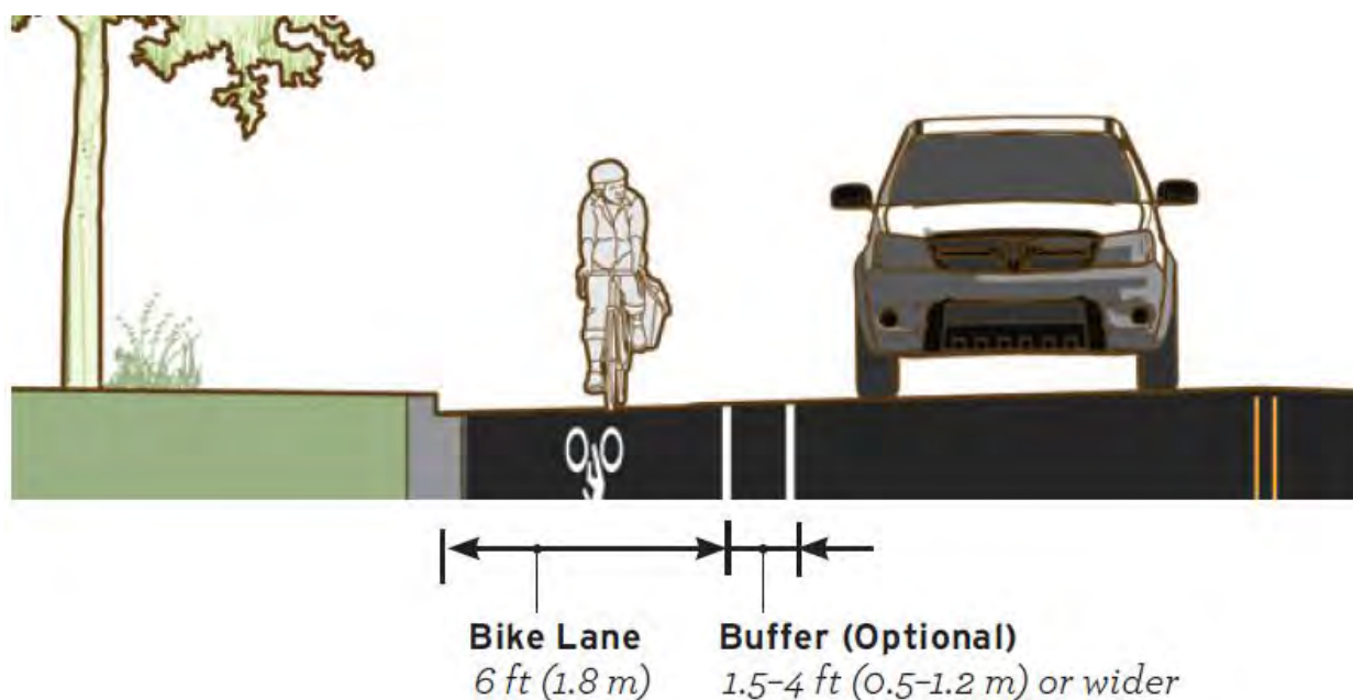
Figure 56: Adequate Bicycle Lane Width Example (Source: FHWA)
