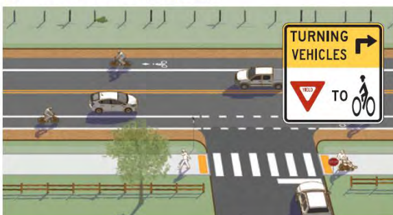
Figure 55: Proper bicycle lane striping at a side street intersection (Source: FHWA)
