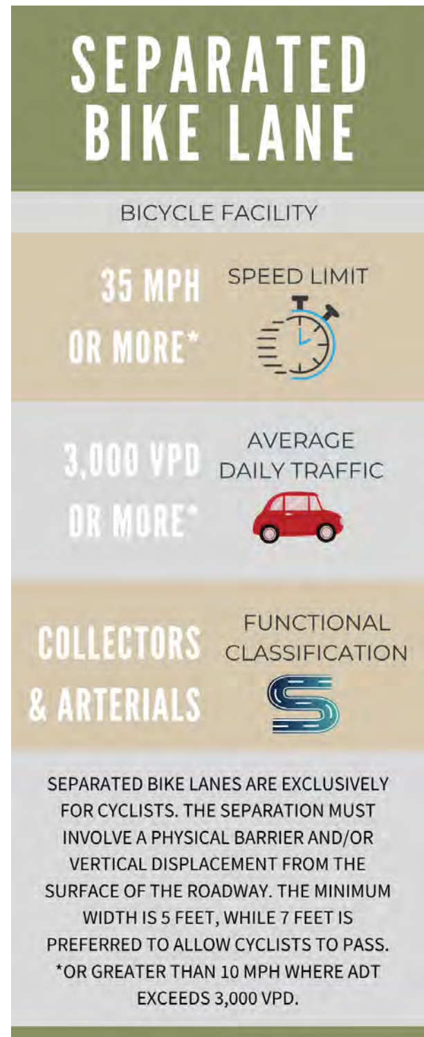
Figure 46: Separated Bike Lane Guidance
