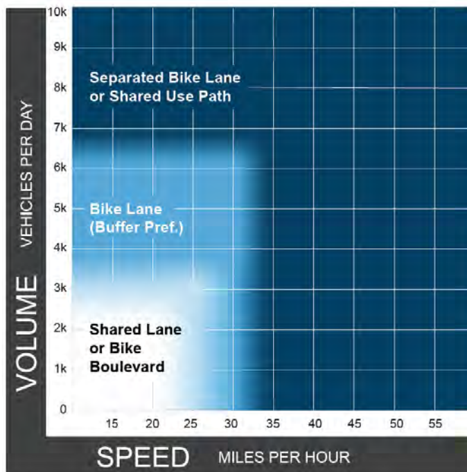
Figure 41: Preferred Bikeway for Urban, Suburban, and Rural Town Streets (Source: FHWA)
