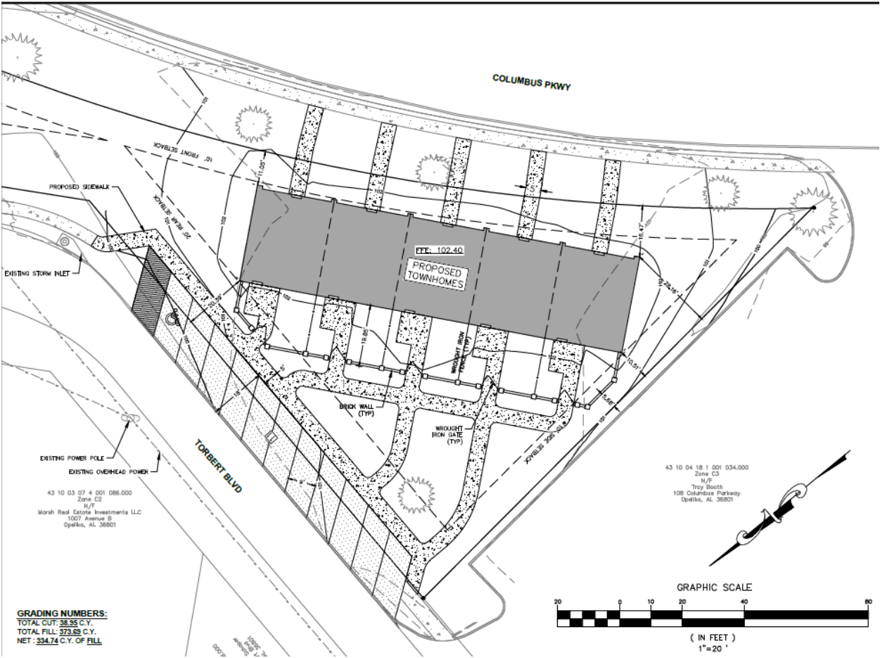
Proposed site plan showing tree placement and parking will be in rear off Tolbert Blvd
